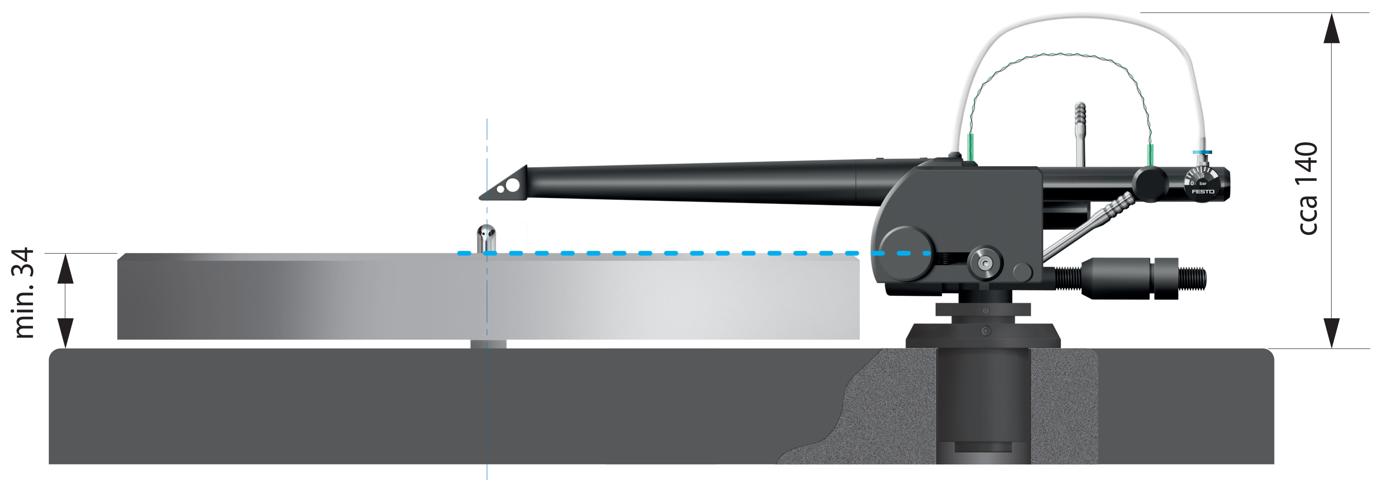
KUZMA Air Line Tonearm Side view
