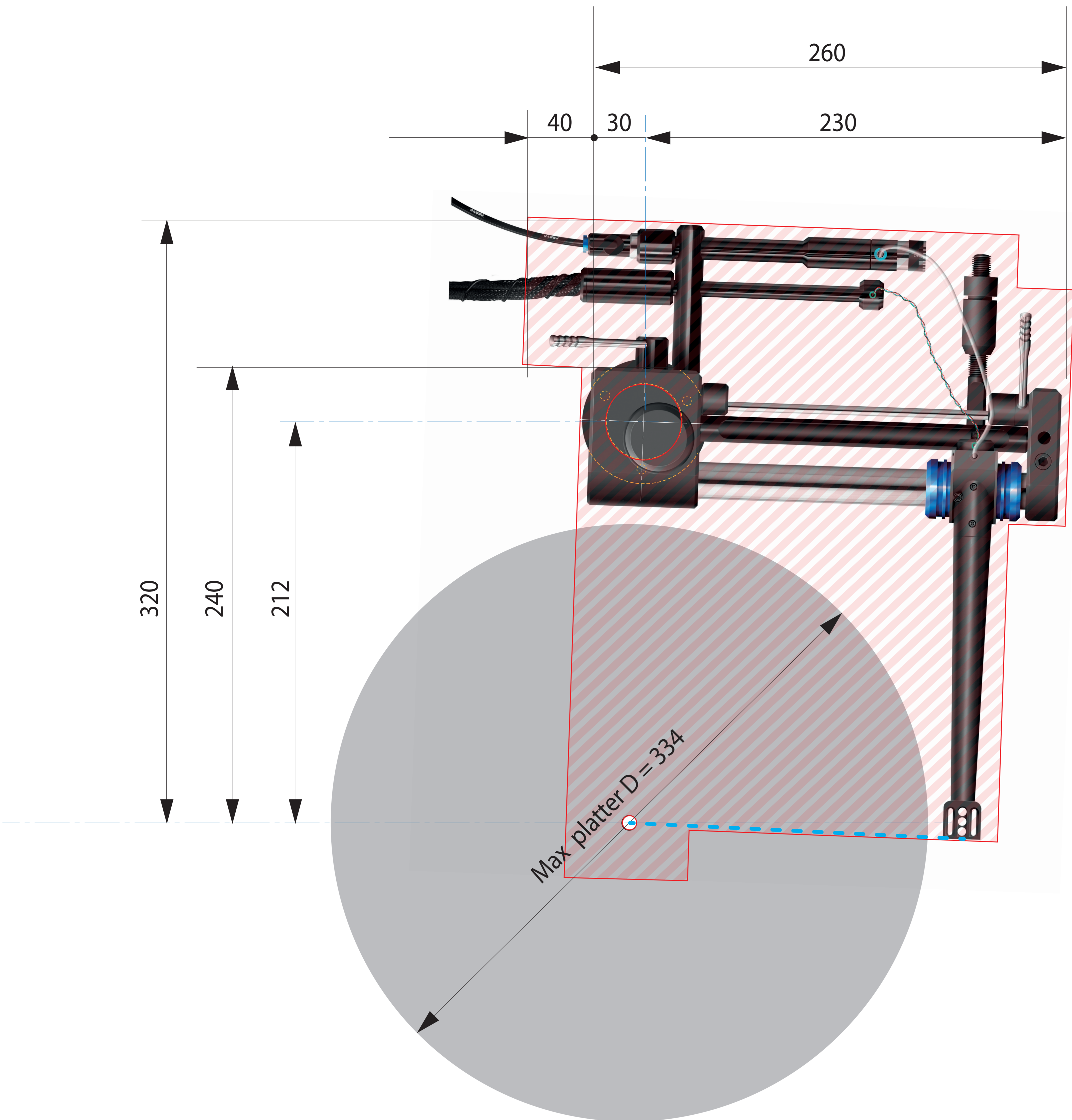
KUZMA Air Line Tonearm Top view
