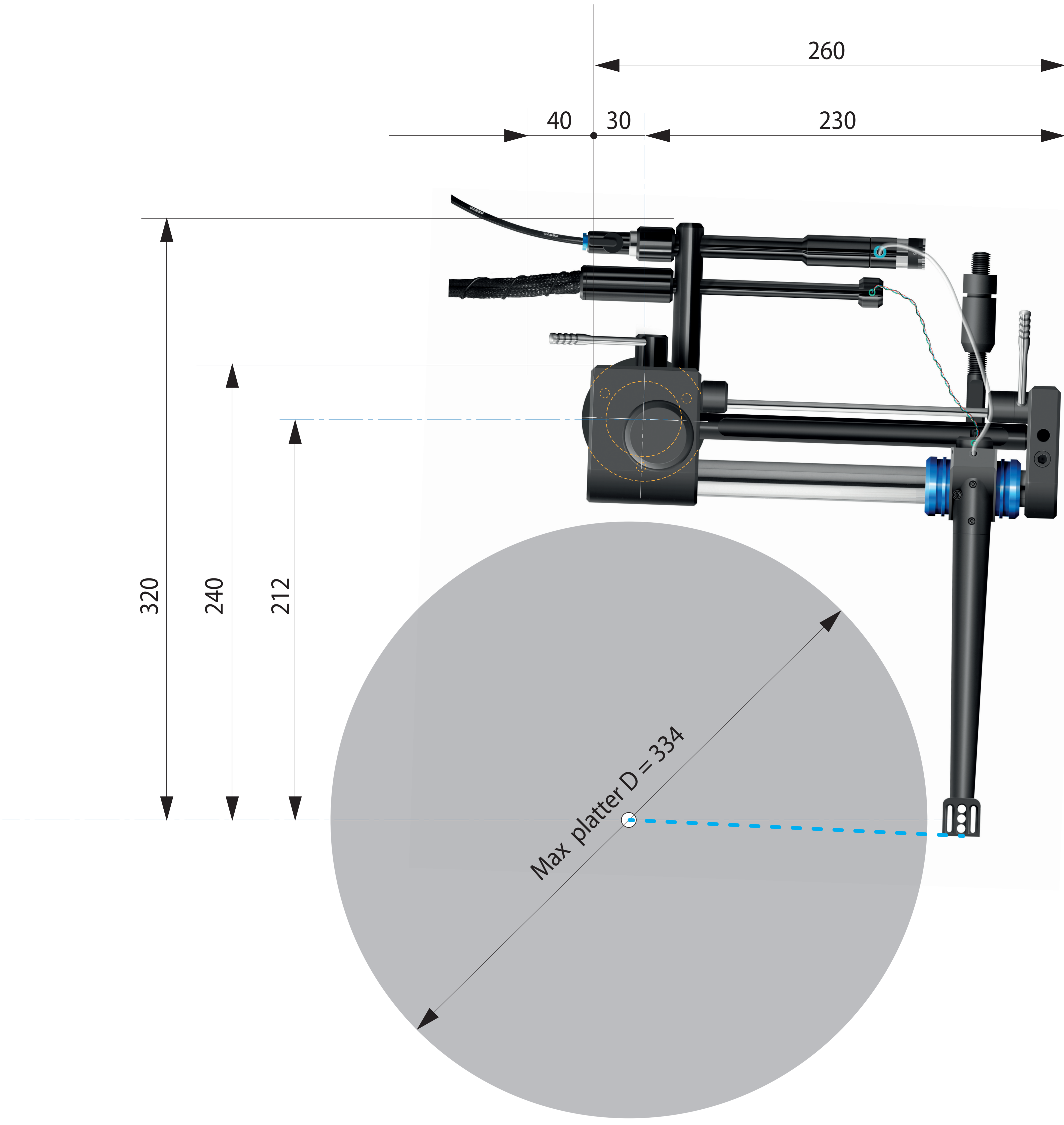
KUZMA Air Line Tonearm Top view
