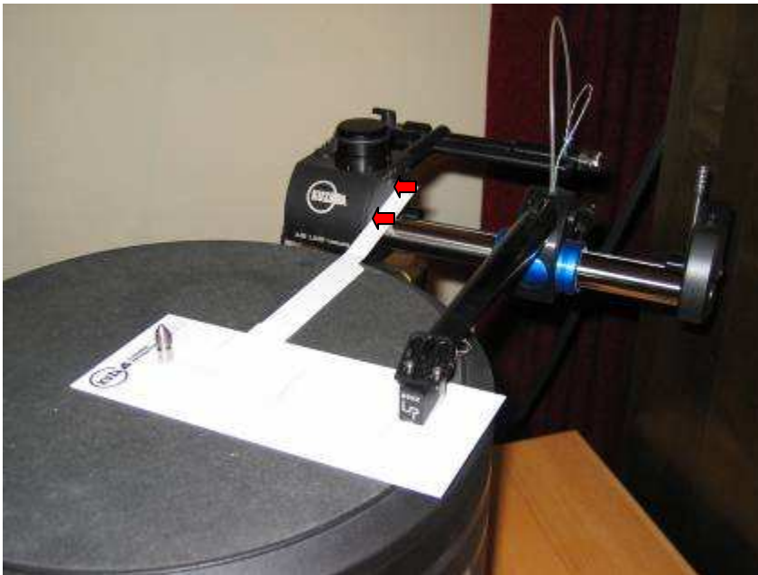
Protractor position
