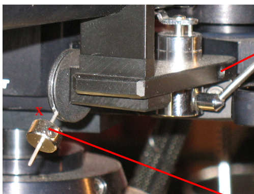
Fig. 9 Bias adjustment
