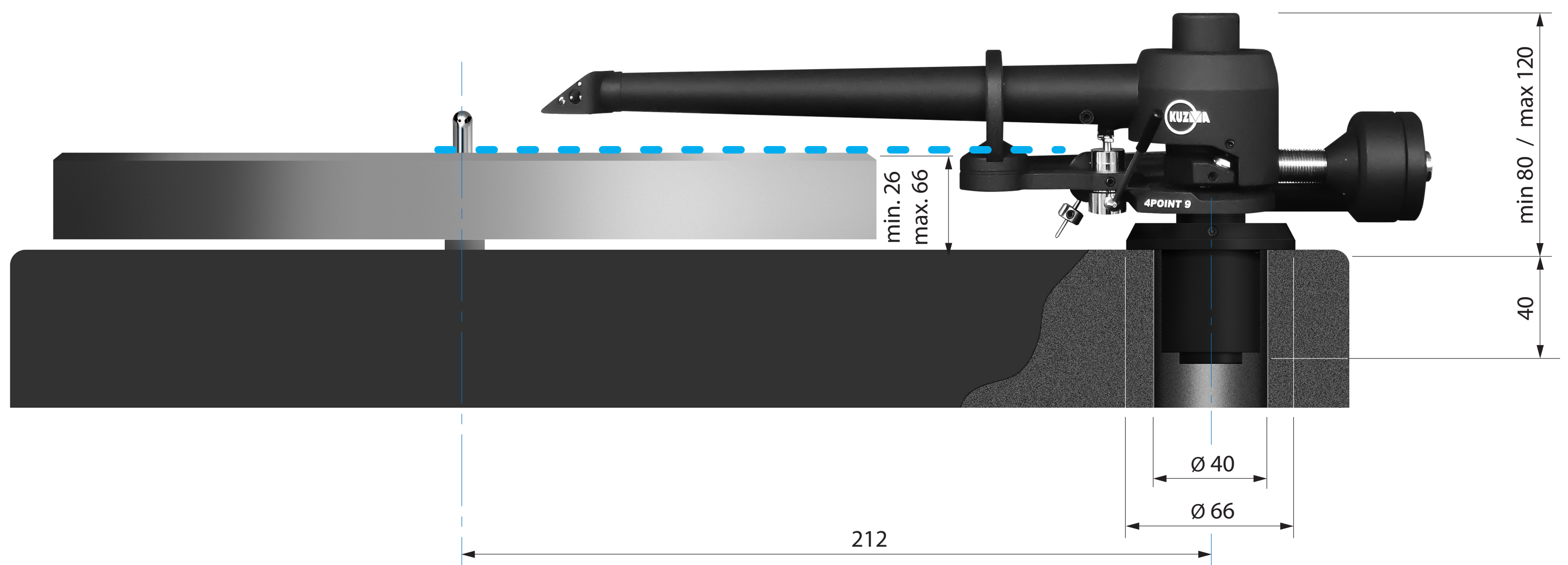
KUZMA 4Point 9" Tonearm Side view
