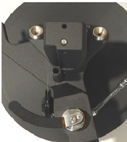
Fig. 8a. Arm tower with square top
