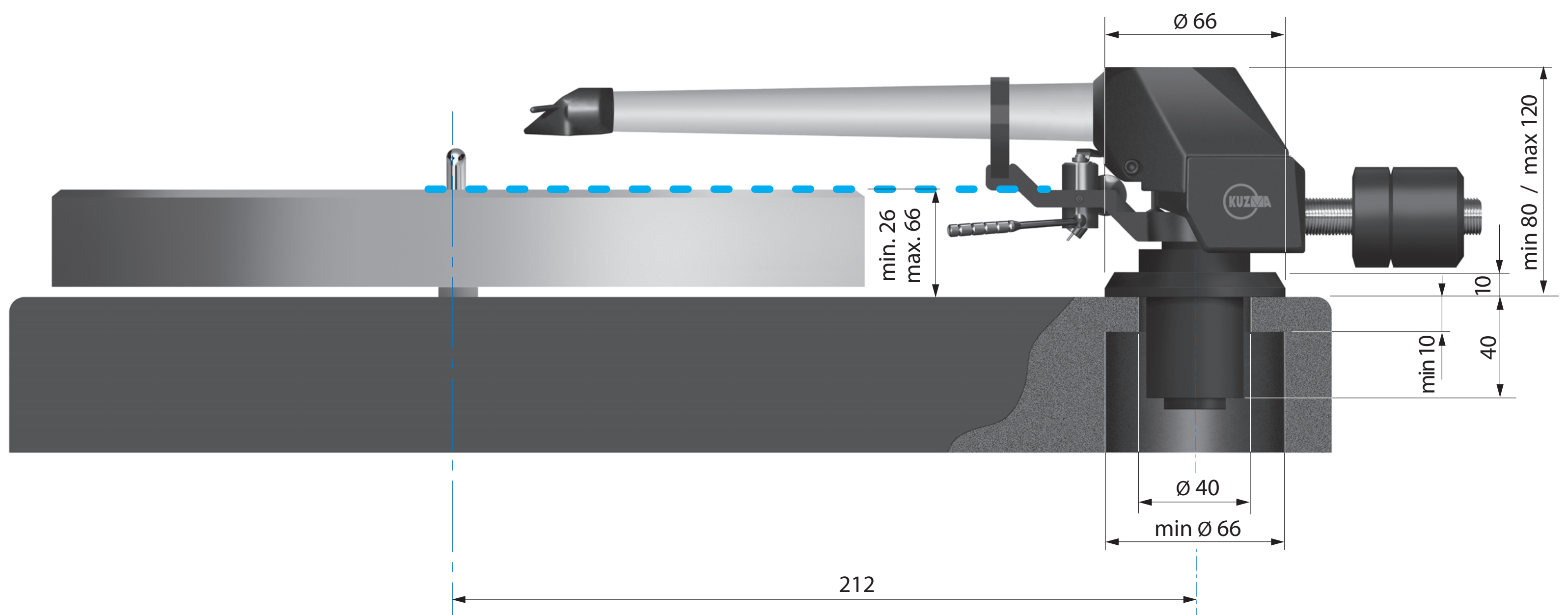
KUZMA Safir 9" Tonearm Side view
