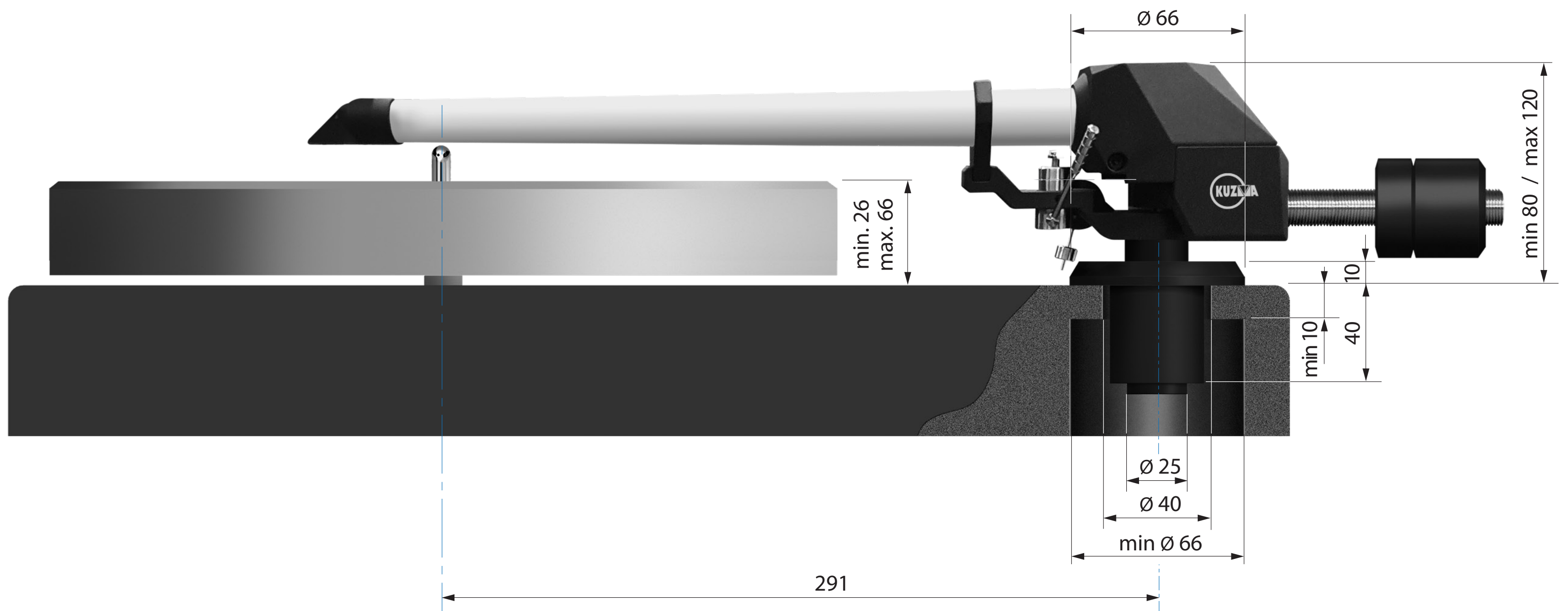
KUZZA Safir 12'' Tonearm Side view
