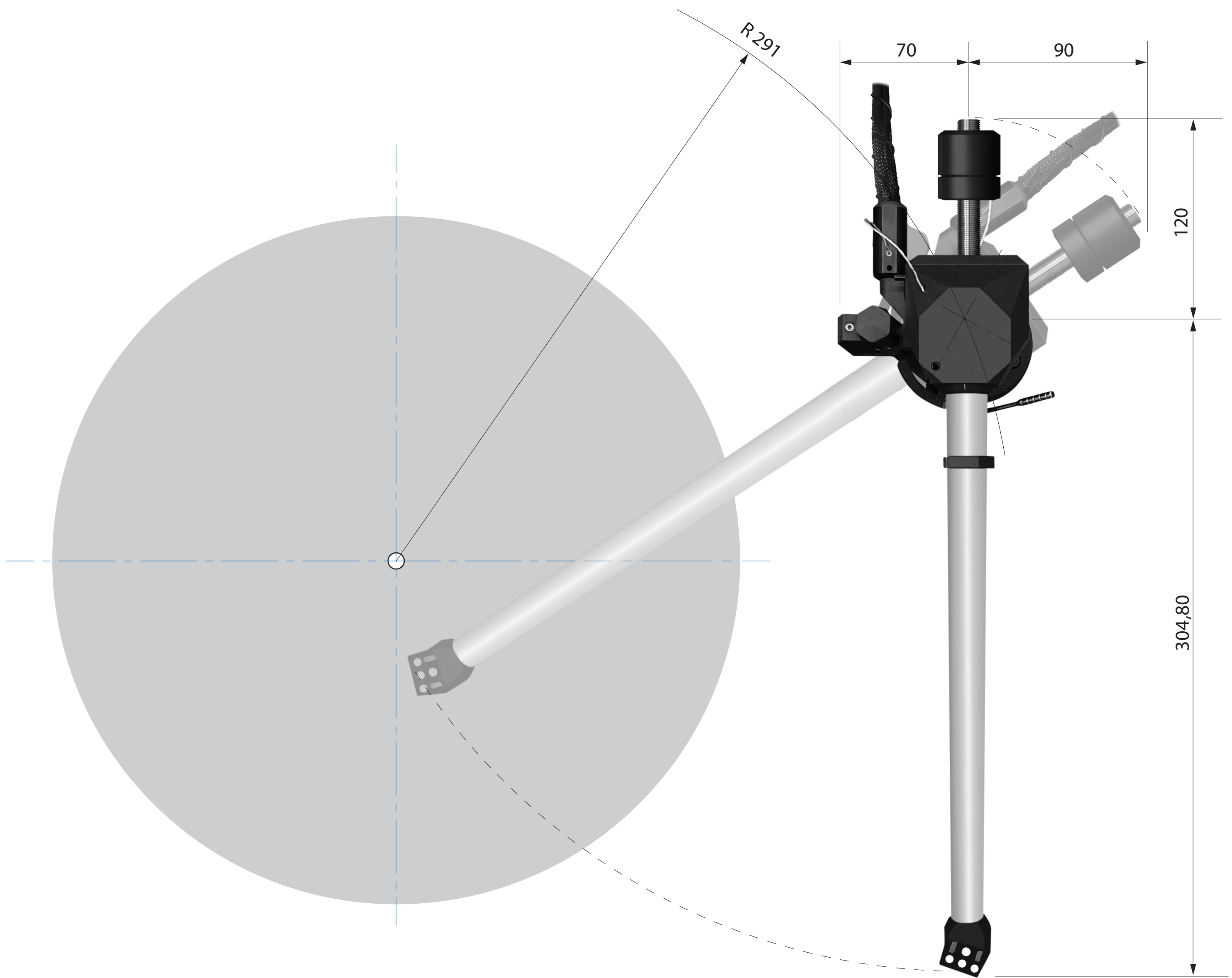
KUZZA Safir 12'' Tonearm Top view
